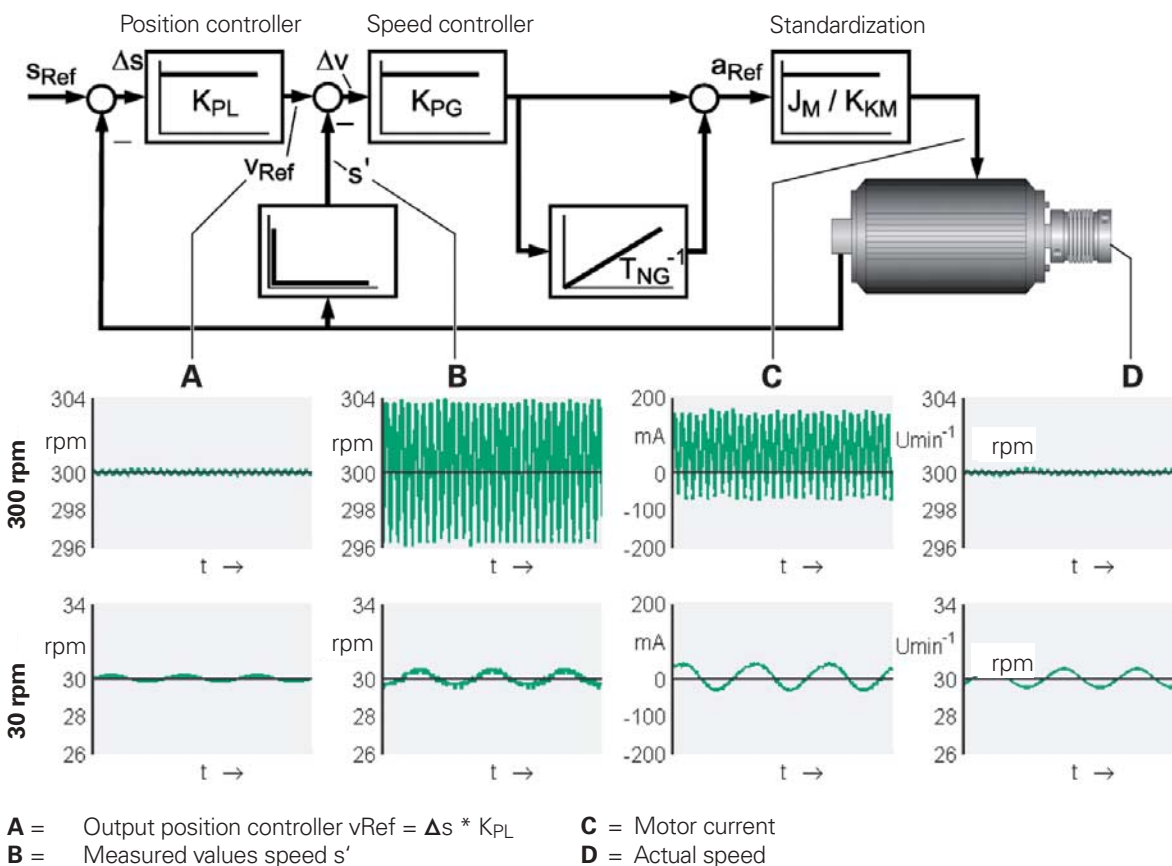
Figure 1: Effect of the interpolation errors in the control loop of a servo drive at two different speeds
